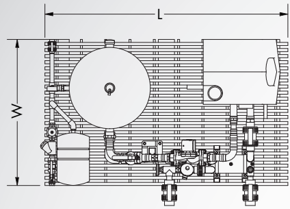
PLAN VIEW ABP-110 ~ 285
